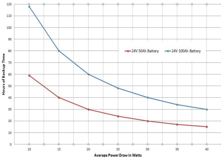
Backup Time vs Average Power Draw
