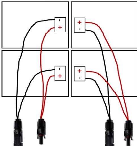
12V Four Panel Configuration
