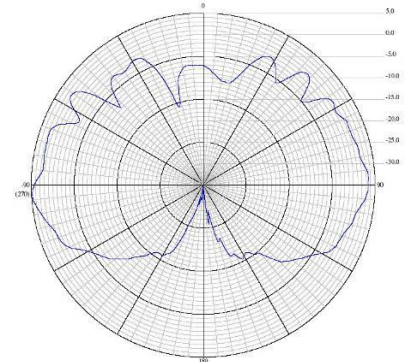
Elevation Pattern 5725 MHz
