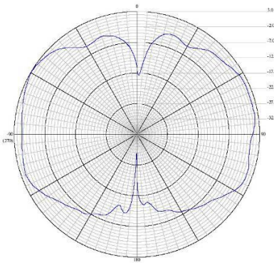
Elevation Pattern 2450 MHz
